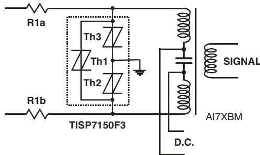
Figure 37. ISDN Protection
