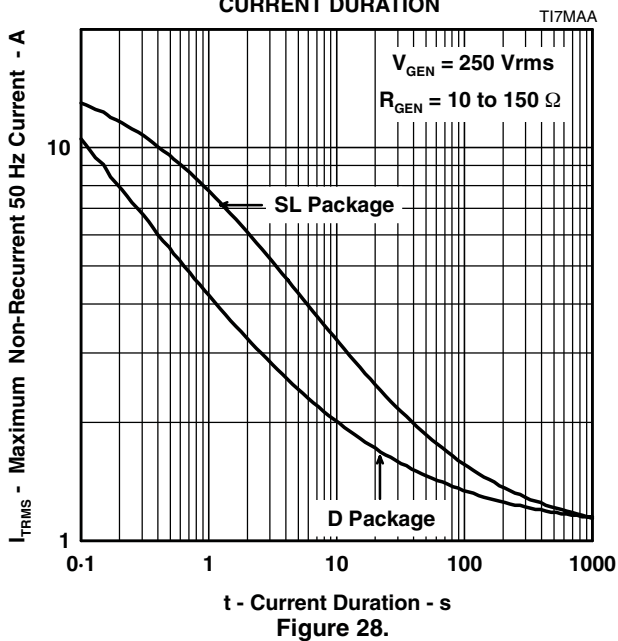
TISP7125F3 THRU TISP7180F3 MAXIMUM NON-RECURRING 50 Hz CURRENT vs CURRENT DURATION
