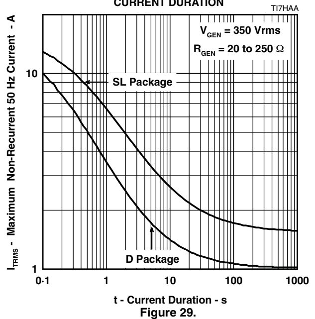
TISP7240F3 THRU TISP7380F3 MAXIMUM NON-RECURRING 50 Hz CURRENT vs CURRENT DURATION
